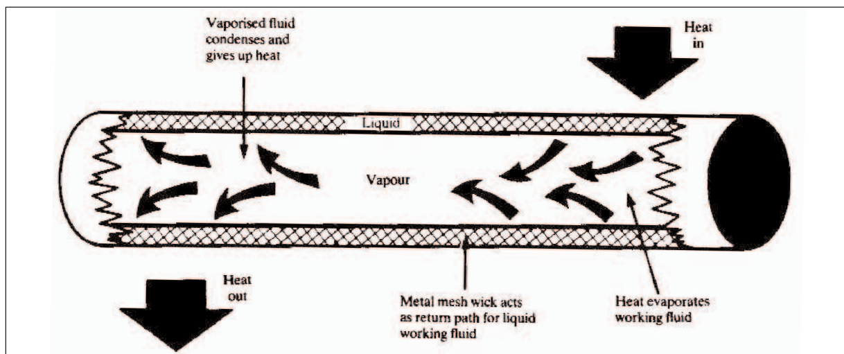
Figure 8.7 Heat Pipe
