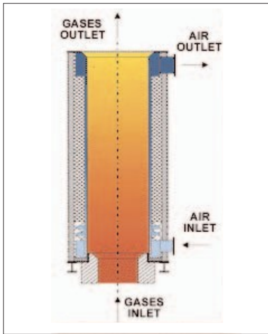
Figure 8.2 Metallic Radiation Recuperator
