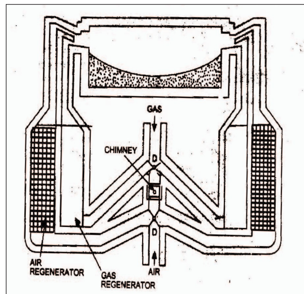
Figure 8.5 Regenerator
