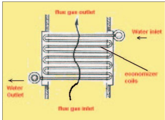
Figure 8.8 Economiser
